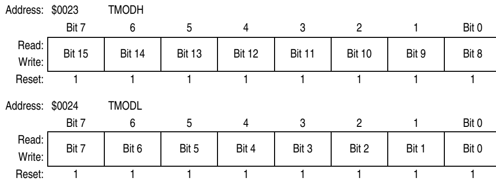
Figure 14-6. TIM Counter Modulo Registers (TMODH:TMDL)
