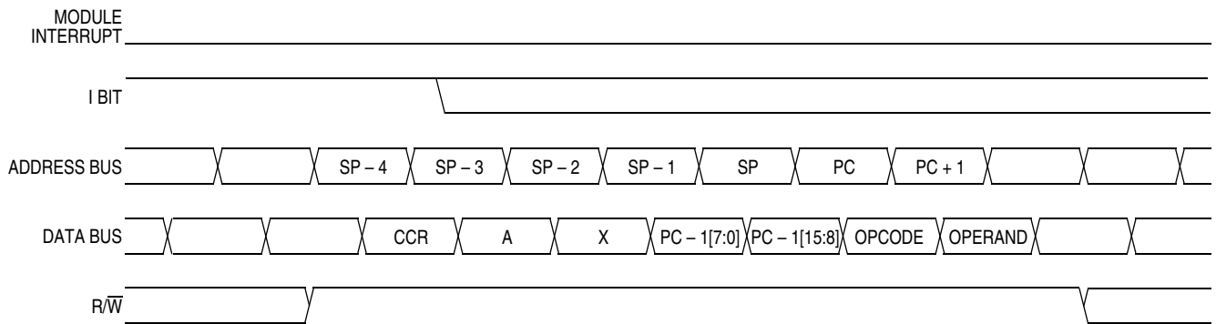
Figure 13-9. Interrupt Recovery
